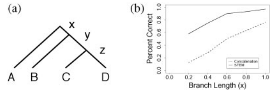
Fig. 1. (a) Model tree used for the simulations; (b) Results of the simulations comparing the performance of STEM to concatenation in terms of the percent of times the true species trees is obtained as a function of x .
